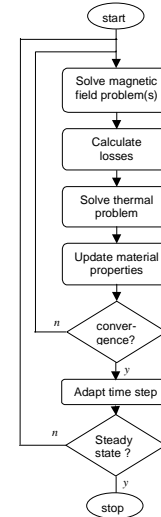
Fig. 4. Coupled problem computation flow chart.
