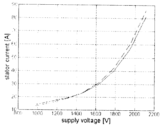
Fig. 2. Calculated and measured no-load characteristic.
