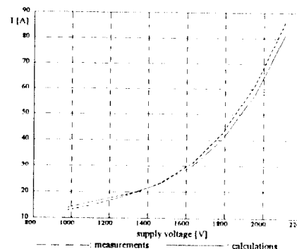
Fig. 1: Calculated and measured no-load characteristic.
