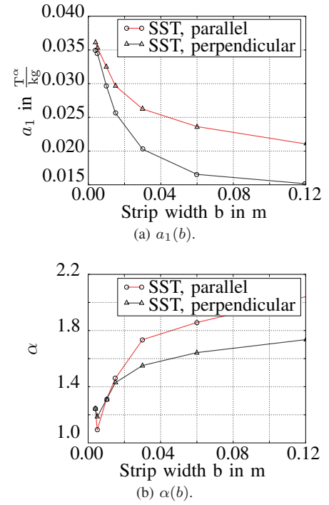
Fig. 4: Identification of (a) a_1(b) and (b) \alpha(b) the hysteresis loss parameter dependent on the strip width.
