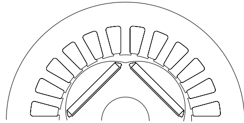
Fig. 1: Cross section of the machine geometry.
