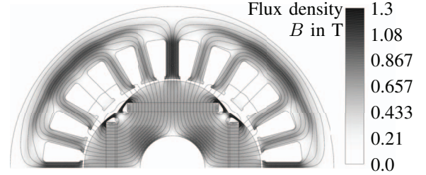
(b) CE affected solution considering the continuous material model.
