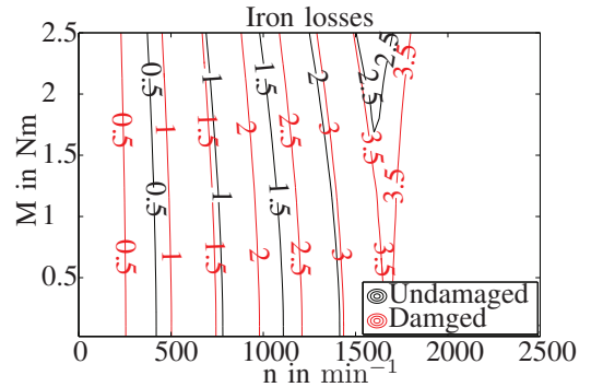
(a) Resulting iron losses.
