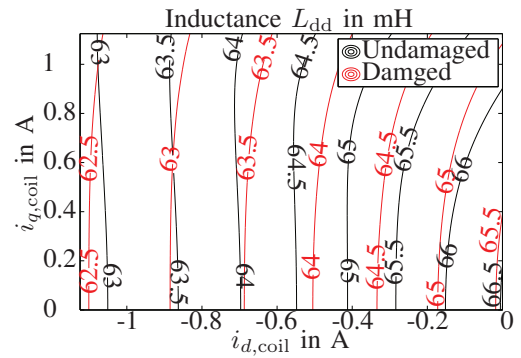
(b) Resulting main inductance in magnetic d-axis.
