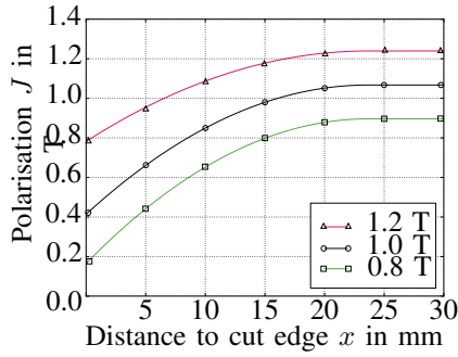
Fig. 2: Local magnetic polarisation J at different mean flux densities.
