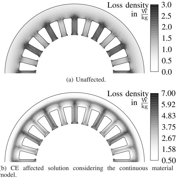
Fig. 5: Local hysteresis loss density distribution in an exemplary working point considering (a) an unaffected and (b) a CE affected material behaviour on the stator geometry.
