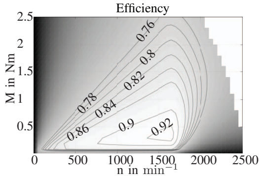
(a) Unaffected material characteristic.
