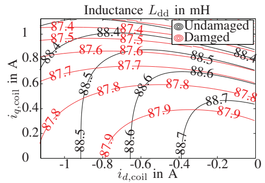
(c) Resulting main inductance in magnetic q-axis.
