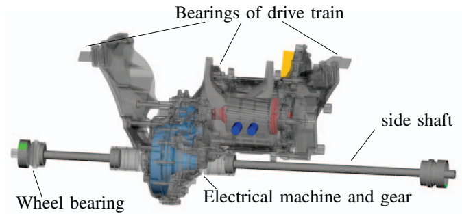
Figure 12. Structure dynamic model of the drive train, including electrical machine, gear, differential, side shaft, wheel bearings and supporting arms, to adapt the drive train in the chassis. Dynamic simulation of the structure behavior is performed, depending on the force excitation entry, which is presented in section III.
