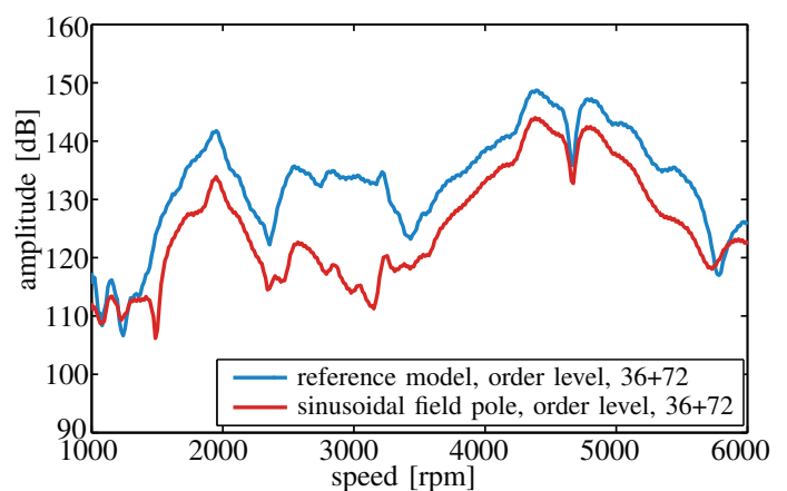
Figure 13. Order level for the surface acceleration. Simulation point at the side bearing, connecting the drive train with the chassis of the vehicle. Dominant orders 36 and 72 filtered. Resonance of the machine measurements (Fig. 10) at 3100rpm is not identified at this position. Simulation for reference model (blue line), which is placed in the original electric vehicle and for sinusoidal field pole model (red line), which is a variation to improve acoustic behavior by designing the rotor of the electrical machine.
