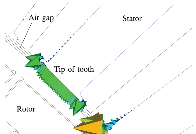
Figure 6. Force density distribution on stator teeth of electrical machine. Node based calculation for every node on the surface of the stator (spatial dependency). Calculation for k = 120 simulation steps with step width \theta_{\text{step}} = 0.5^\circ ( 60^\circ part model of the machine for reasons of symmetry).
