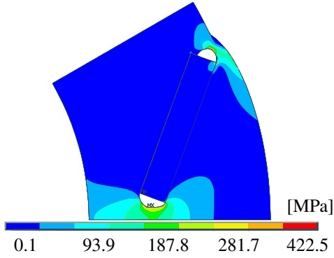
Fig. 7. Centrifugal force simulation for \frac{\delta_q}{\delta_d} = 4 .
