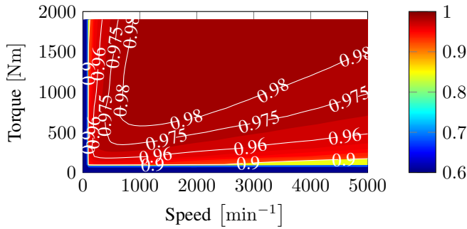
Fig. 4. Efficiency map of the reference VI-PMSM.
