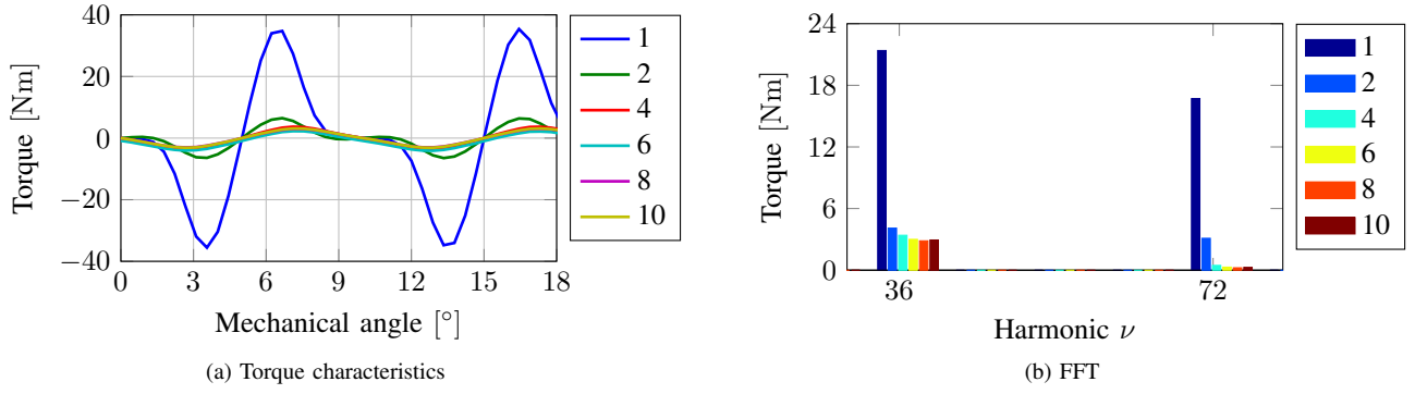
Fig. 8. Cogging torque as a function of \frac{\delta_a}{\delta_d} .
