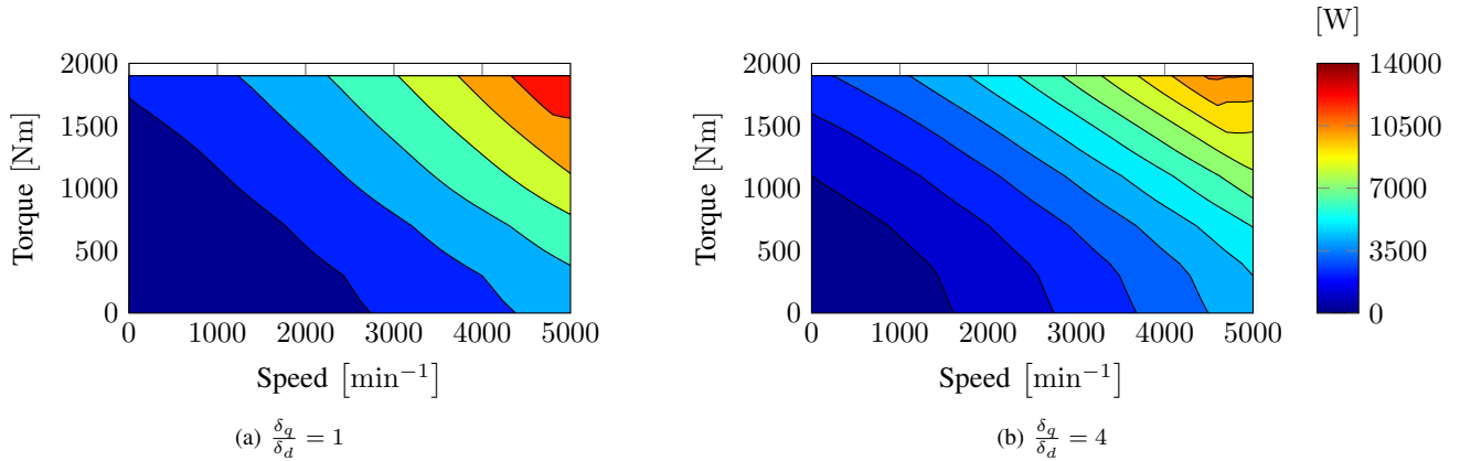
Fig. 10. Total losses for different \frac{\delta_a}{\delta_d} .
