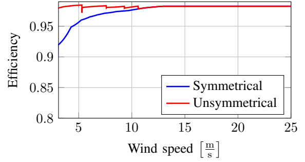
Fig. 5. Symmetrical vs. unsymmetrical power split.
