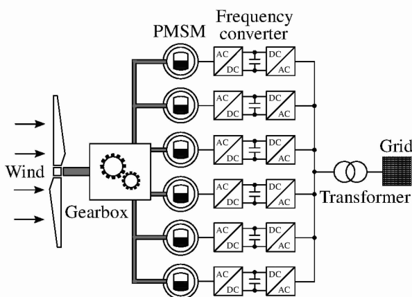
Fig. 2. Schematic diagram of a WT with six high-speed generators.
