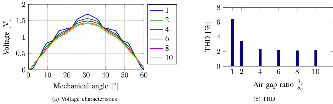
Fig. 9. Induced phase-to-phase voltage as a function of \frac{\delta_a}{\delta_d} .
