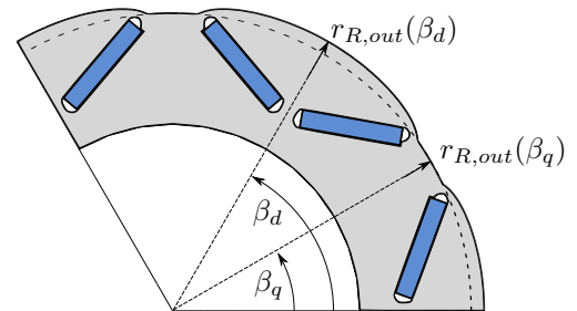
Fig. 6. Model of the VI-PMSM with sinusoidal rotor field poles, \frac{\delta_q}{\delta_d} = 4 .
