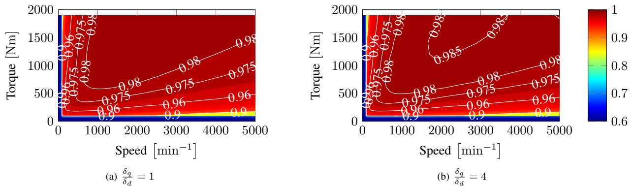
Fig. 11. Efficiency maps for different \frac{\delta_a}{\delta_d} .
