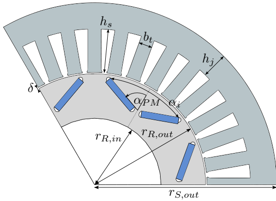
Fig. 3. Geometry model of the reference VI-PMSM.
