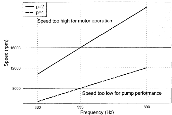
Figure 1: Speed Characteristics.
