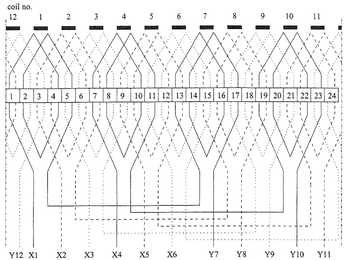
Figure 2: Winding diagram.
