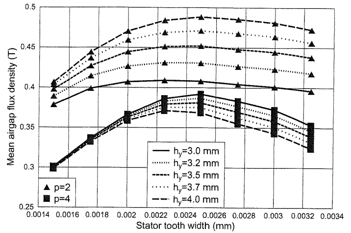
Figure 4: FEM simulation result: Mean airgap flux densities (for p = 4 ; calculated using (12)).
