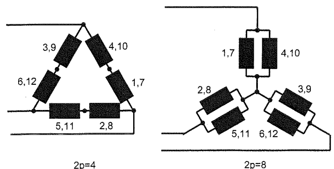
Figure 3: Circuit diagram.
