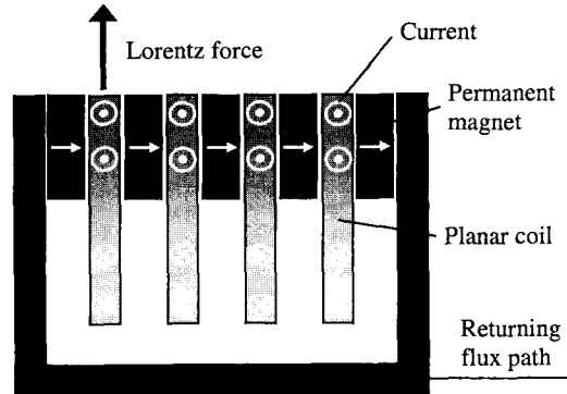
Fig. 13 Principle of 4-in-1 actuator.
