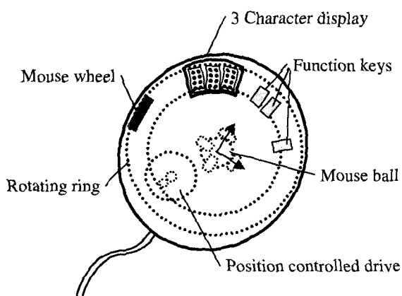
Fig. 4 Design concept of a Braille mouse.
