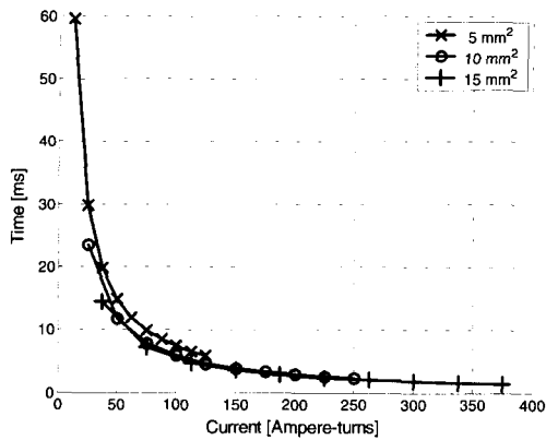
Fig. 23 Time required for an upward displacement of 2 mm. The parameter is the coil section.
