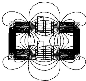
Fig. 24 Flux lines 4-in-1 actuator
