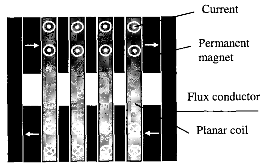
Fig. 14 Design of the 4-in-1 actuator.
