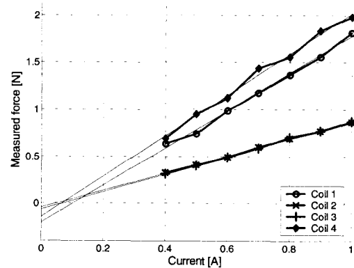
Fig. 28 Measured force as a function of the applied current for all four coils.
