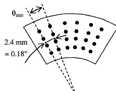
Fig. 15 Position of the pins on the ring.
