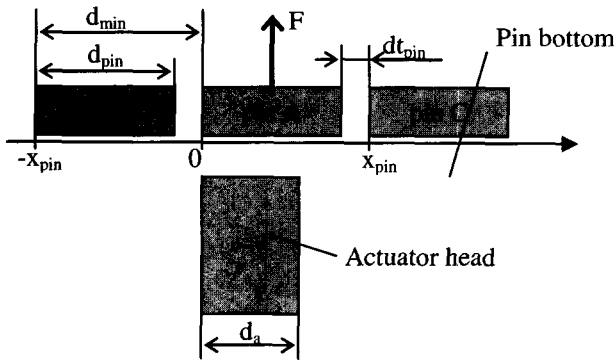
Fig. 16 Position of pins and activation.
