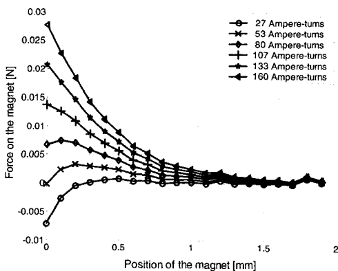
Fig. 20 Force acting on the magnet as a function of the vertical displacement of the magnet. H_c = 200 kA/m; h_{coil} = 10 mm; copper section = 6 mm 2 .
