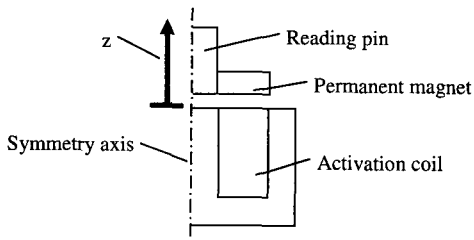
Fig. 19 Model of direct PM actuator.
