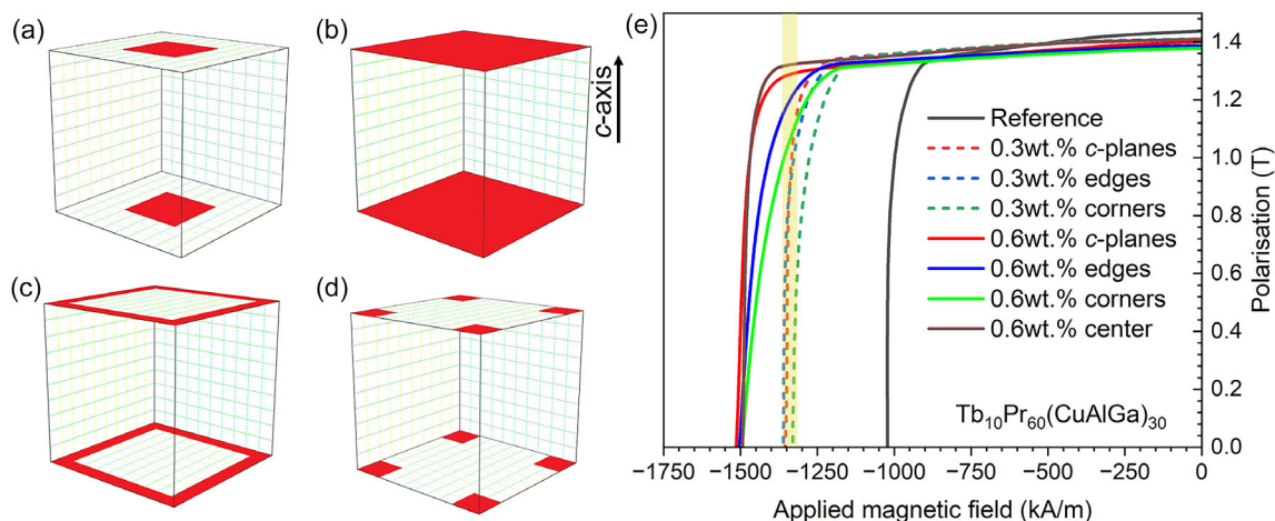
Figure 6. Sketch illustrating HRE application at different locations of the magnet: a) middle of c -planes, b) uniform c -planes, c) edges, and d) corners. The corresponding demagnetization curves after GBDP of 0.3 wt% and 0.6 wt% of \text{Tb}_{10}\text{Pr}_{60}(\text{CuAlGa})_{30} are shown in e). The shaded area in (e) indicates the statistical deviation in coercivity ( \pm 50 \text{ kA m}^{-1} ) after preparation and characterization of multiple samples.
