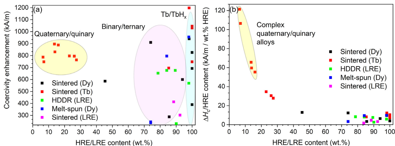
Figure 1. a) Selected literature values for coercivity enhancement by HRE/LRE diffusion in various types of NdFeB magnets. b) The corresponding coercivity enhancement normalized to the RE content showing the efficiency of the different sources.
