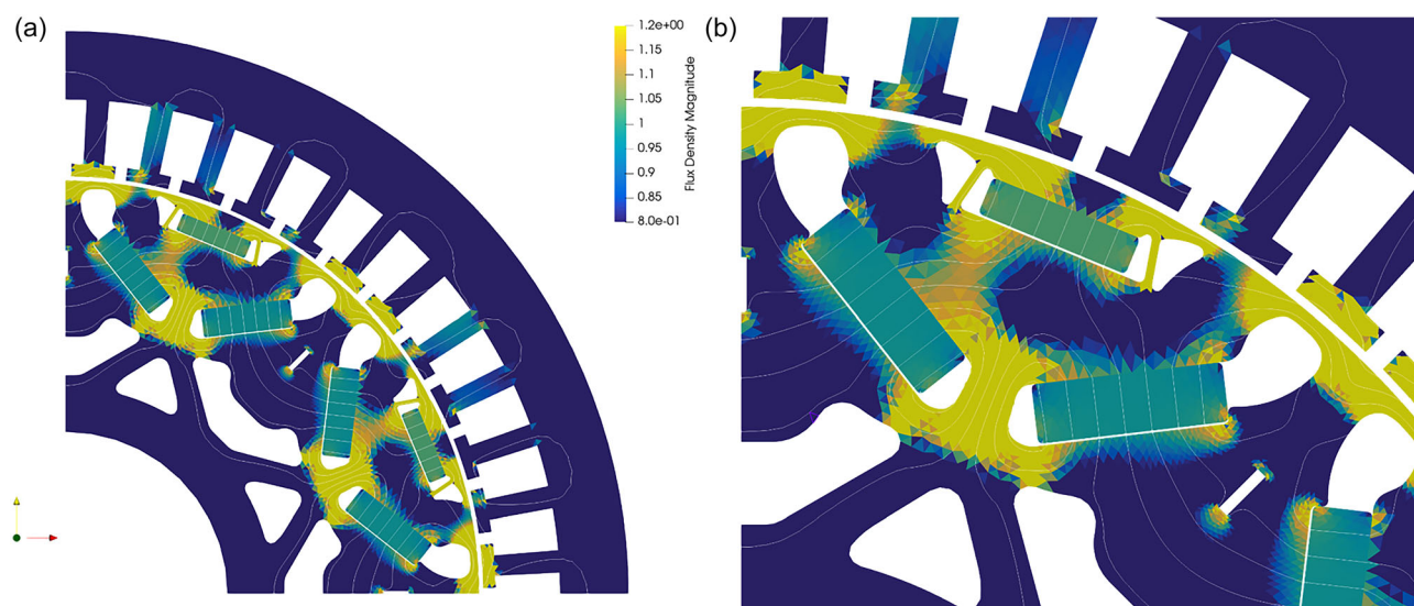
Figure 5. A 2D FE-Simulated flux density distribution for a typical internal permanent magnet synchronous traction motor from electric vehicles in the short-circuit operating point. a) overview of the geometry and b) magnified section showing that the level of demagnetization is not distributed homogeneously with the highest demagnetization occurring at the edges of the inner magnets.
