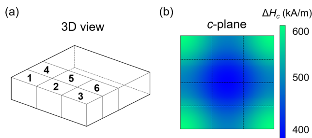
Figure 7. Sketch illustrating coercivity mapping after HRE application on c -planes corners. a) 3D view shows cutting in six cubes for individual local M(H) measurements. b) Color map represents the resultant coercivity enhancement ( \Delta H_c ) mapping constructed from individual measurements illustrated in (a).
