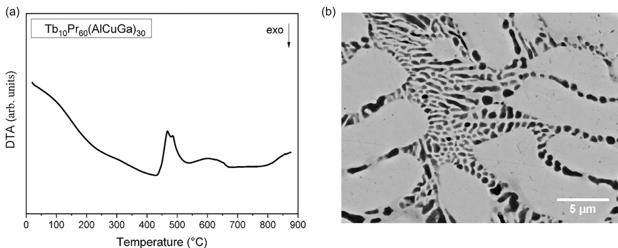
Figure 3. a) DTA heating curve for Tb 10 Pr 60 (Cu,Al,Ga) 30 composition showing multiple endothermic melting events. b) SEM BSE image of the eutectic microstructure for the as-cast alloy.
