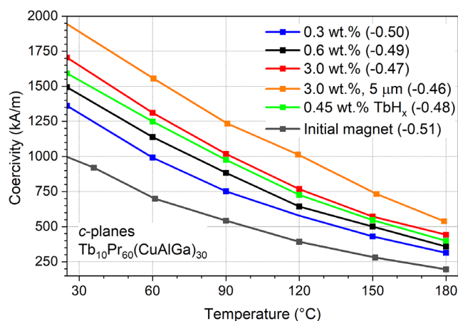
Figure 10. Temperature stability of coercivity for different GBDP sources applied on c -planes. The respective \beta values are given in the parentheses.
