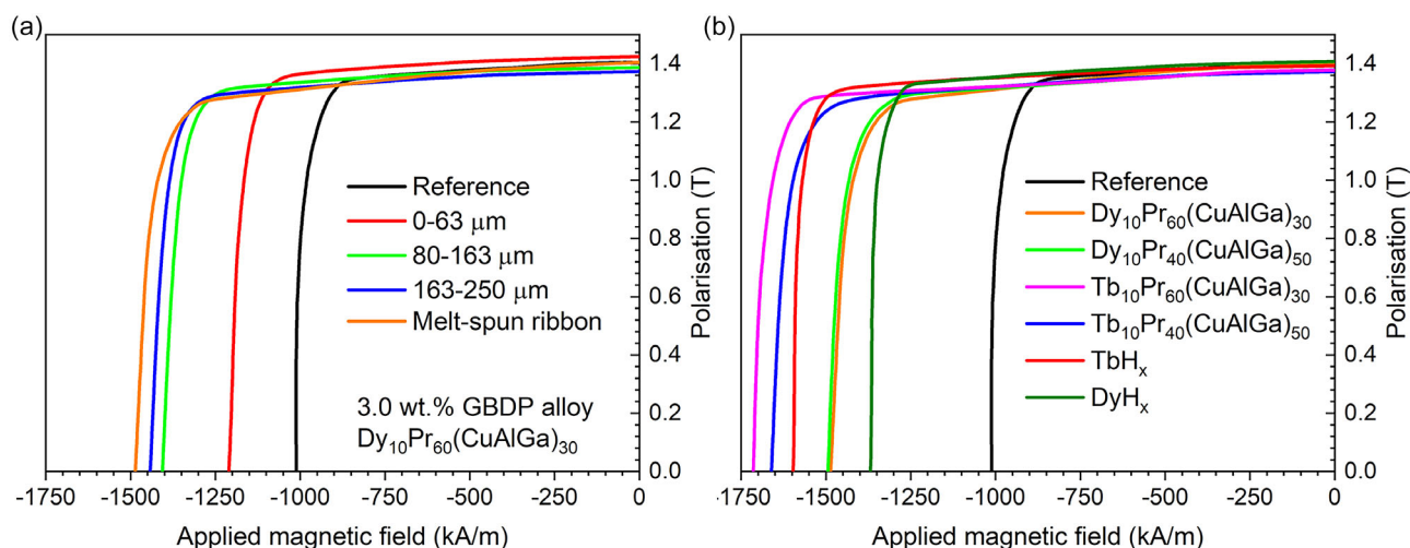
Figure 2. Optimization of GBDP source alloy composition and application form. a) the effect of particle size and b) the effect of composition. 3.0 wt% of GBDP alloy (melt-spun ribbons) and 0.4 wt% HRE hydrides (powder) were used for equal HRE usage.
