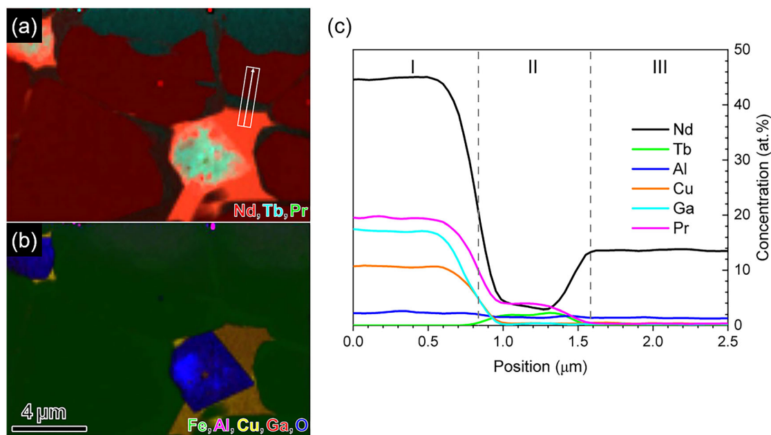
Figure 9. STEM-EDS elemental maps for a) Nd, Tb, Pr and b) Fe, Al, Cu, Ga, O. Elemental concentrations line profiles across the indicated arrow are presented in c).
