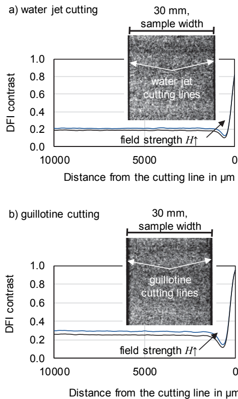
Fig.5 DFI contrast images from NGI measurements and top view images of samples processed with a) water jet cutting, 3.5 Å wave-length and b) guillotine cutting 3.2 Å wave-length, at two field strengths
