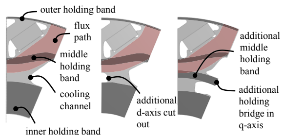
Fig. 8. Three different approaches for weight reduction
