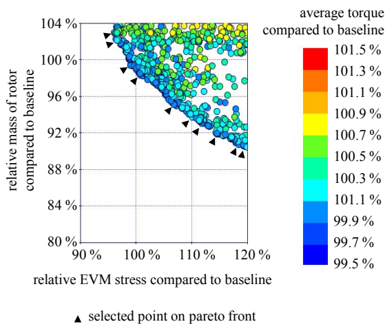
Fig. 10. Results of Pareto optimization for cooling channel and selection of points on Pareto front for comparison
