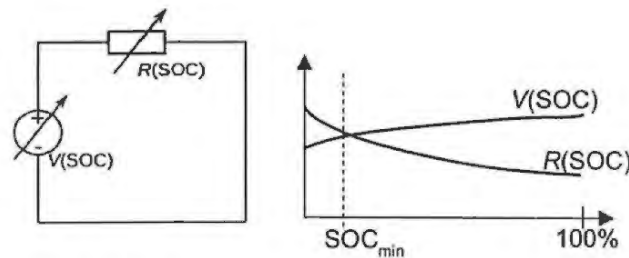
Figure 1: Battery equivalent circuit in this paper.
