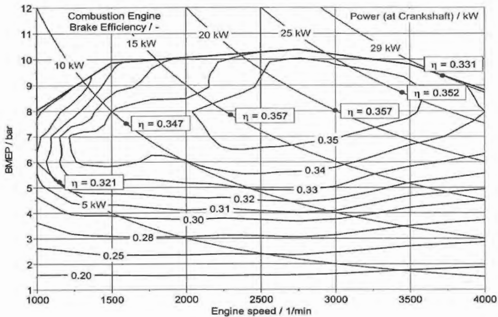
Figure 2: Brake efficiency of the advanced engine
