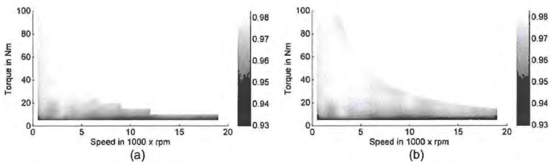
Figure 3: Efficiency map of the transmission obtained from (a) experiments (b) surrogate model.
