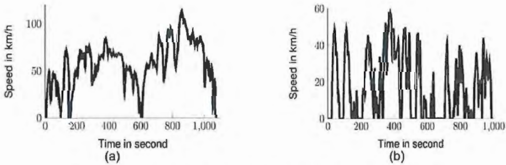
Figure 6: Speed profile of Artemis driving cycle (a) Rural (b) Urban.
