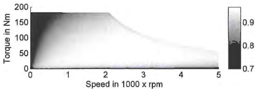
Figure 4: Efficiency map of the direct driven generator.
