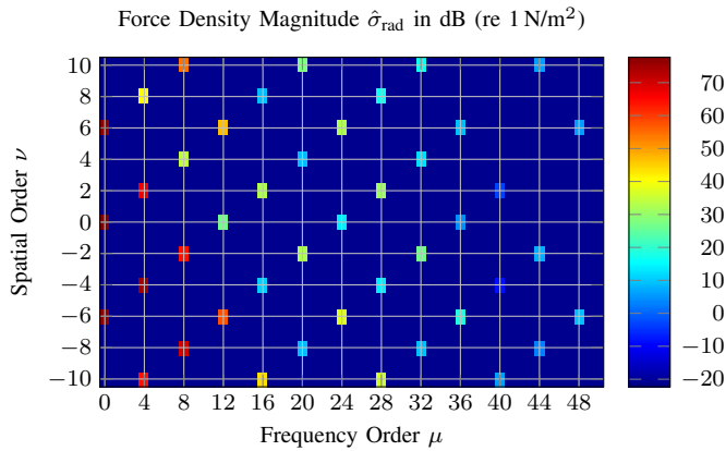
Fig. 14. Radial force density magnitudes for a six teeth and four poles surface mounted PMSM without manufacturing tolerances as a function of spatial order \nu and frequency order \mu .
