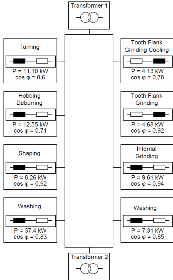
Fig. 2.4.8 Schematic power grid of the production line
