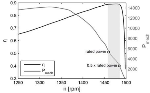
Fig. 2.4.6 Efficiency and mechanical power of a 5.5 kW induction machine
